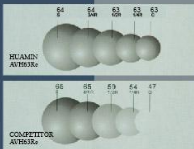
Sectional view for measuring points in a steel ball
