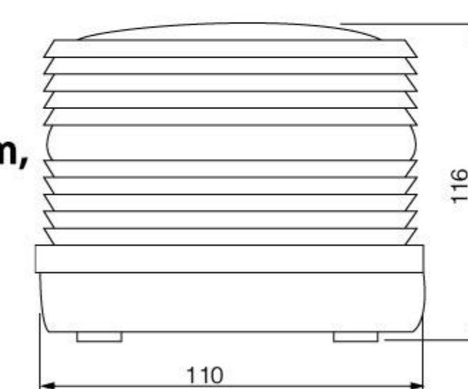
尺寸线图 Dimensional line diagram
