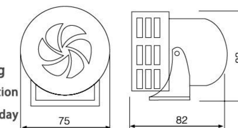
尺寸线图 Dimensional line diagram
