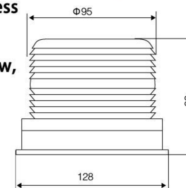
尺寸线图 Dimensional line diagram
