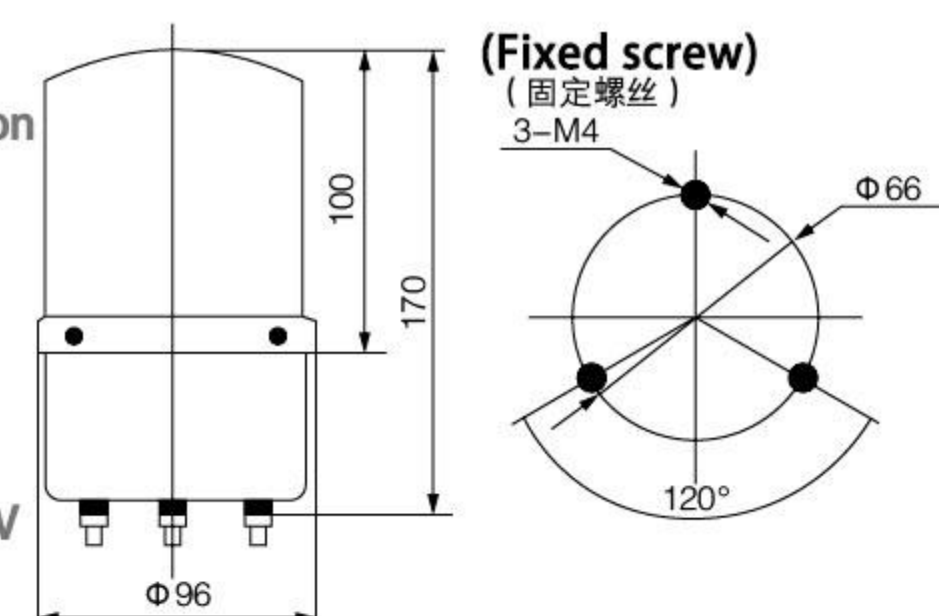
尺寸线图 Dimensional line diagram
