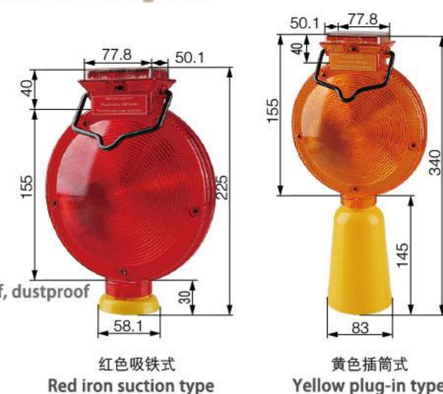
尺寸线图 Dimensional line diagram
