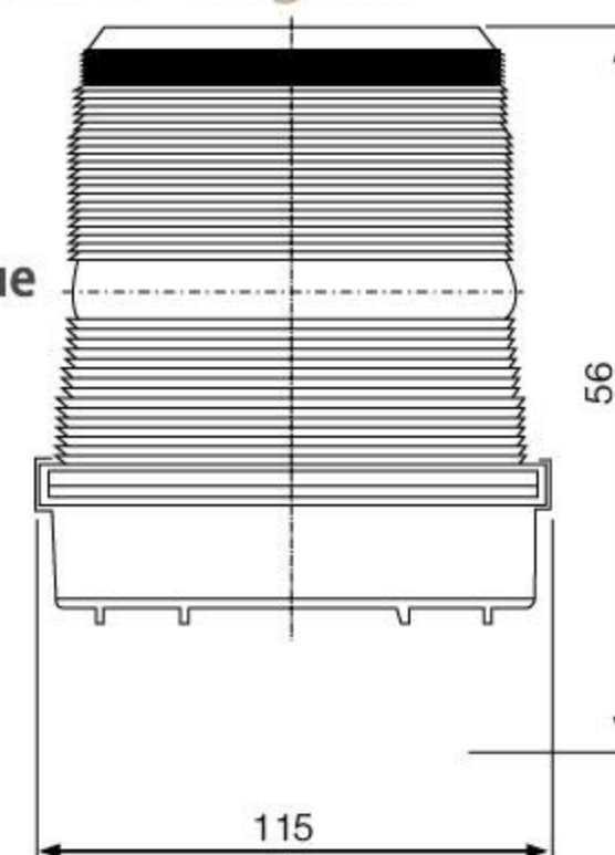
尺寸线图 Dimensional line diagram
