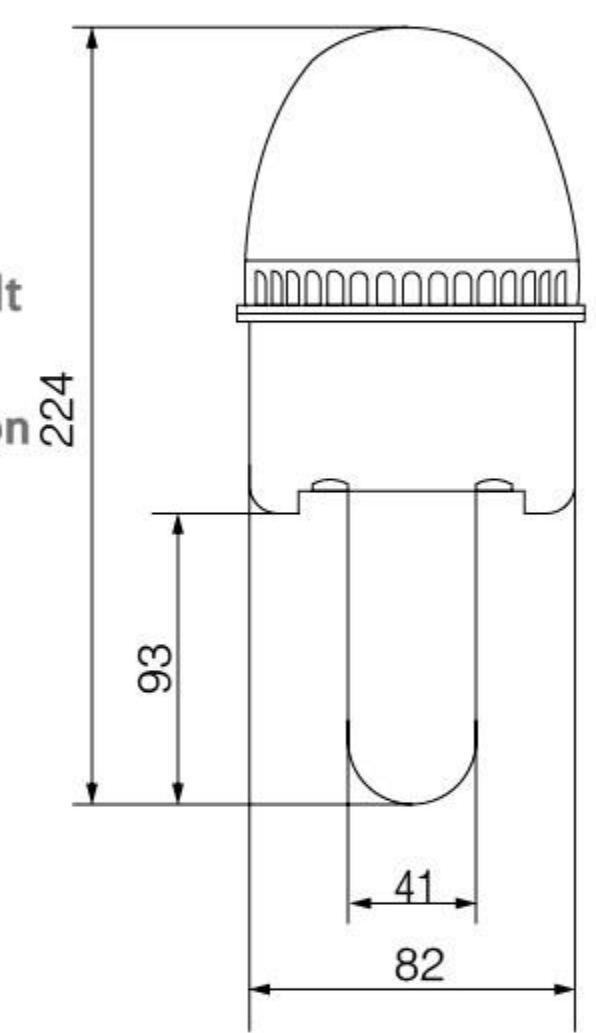
尺寸线图 Dimensional line diagram
