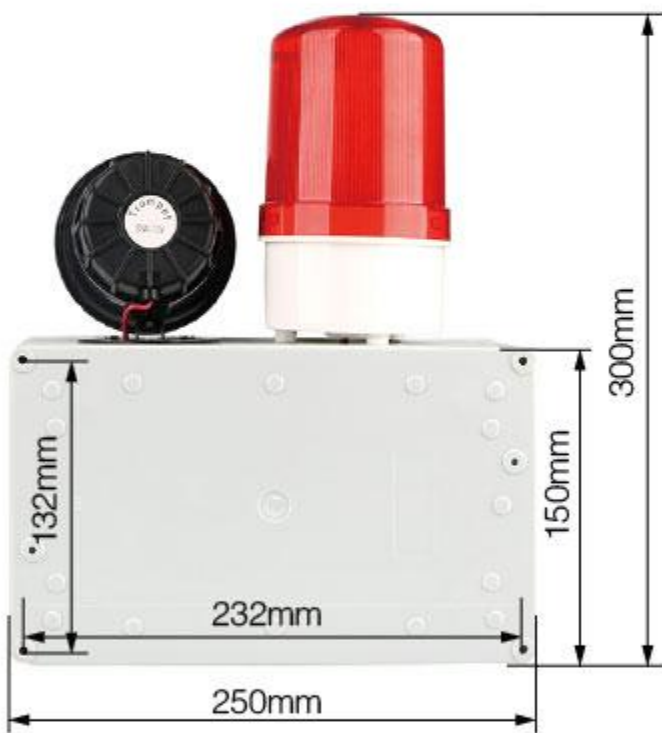
Dimensional line diagram 尺寸线图
