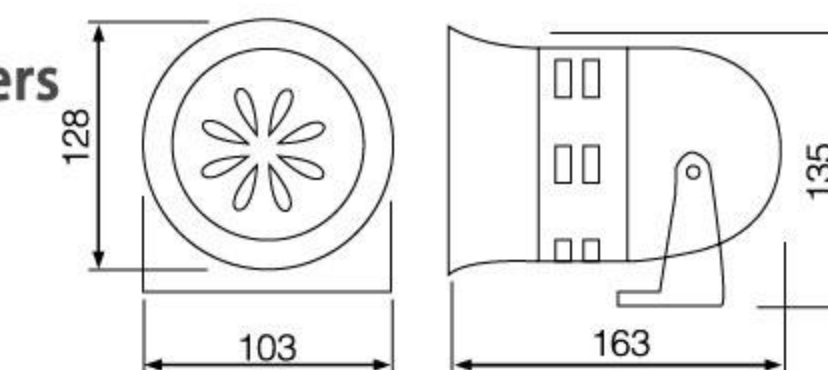
尺寸线图 Dimensional line diagram
