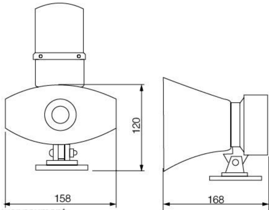
Dimensional line diagram 尺寸线图
