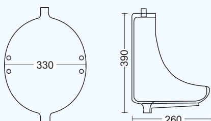
SP-409 | FLAT BACK URINAL
