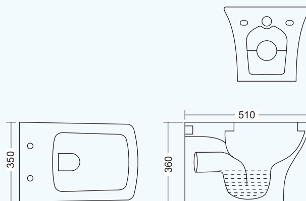
SP-301 FLOOR MOUNT
