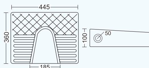
SP-410 | LADIES URINAL
