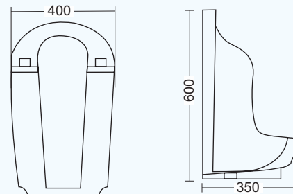
SP-408 | HALF STALL URINAL
