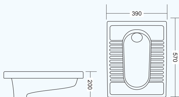
SP-422 ORISSA PAN (20") L 570 W 390 H 200mm
