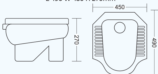
SP-432 | CHINA PAN
