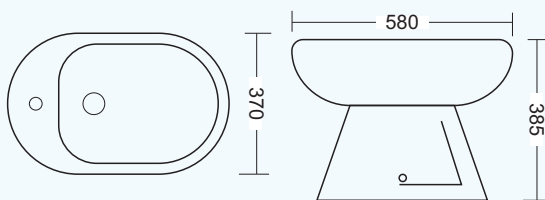
SP-407 | BIDET L 580 W 370 H 385mm
