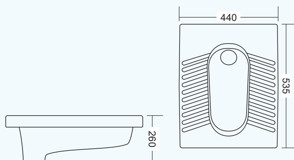
SP-421 DELUXE ORISSA PAN (20") L 535 W 440 H 260mm
