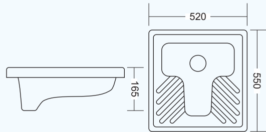
SP-431 | TURKIS PAN
