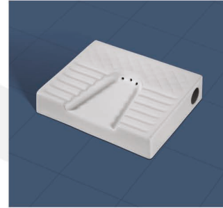
LADIES URINAL (6004) L-360, W-440, H-100mm 14.2 x 17.3 x 4 inch
