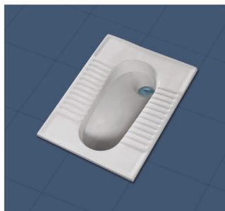
20" ORISSA PAN L-535, W-450, H-265mm
