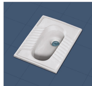
20" CT PAN L-535, W-435, H-160mm
