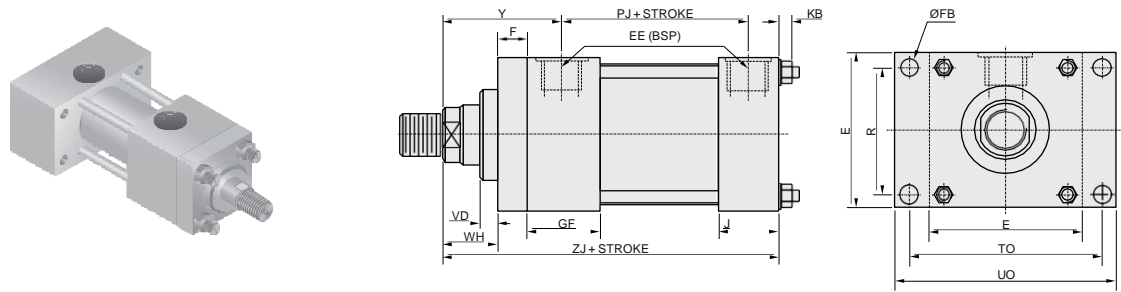
Style 2-Cap Rectangular Flange Mounting
