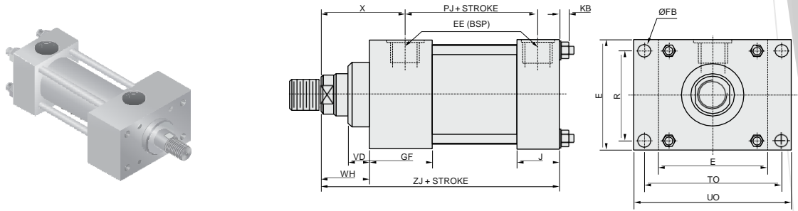
Style 1-Head Rectangular Flange Mounting
