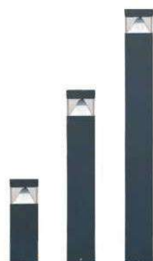
PRODUCT CODE 1628 FILLET POWER 10W, 15W, CCT 3000K, 4000K, 6000K MATERIAL TYPE M.S/ S.S / ALUMINIUM POWDER COATED HEIGHT 600 MM, 900MM, 1200 MM MRP
