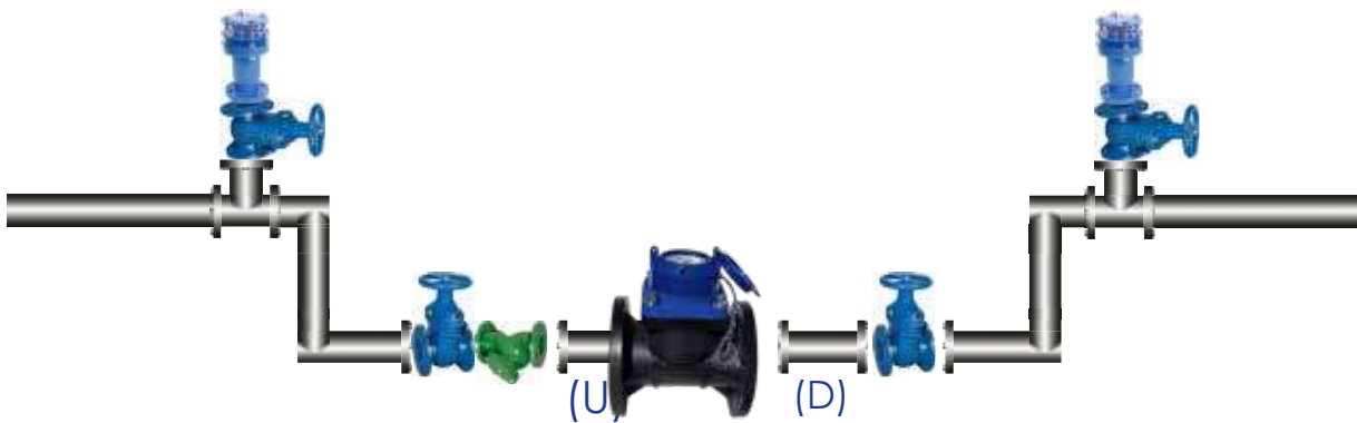
Counter Application Example for 50 -100 mm
