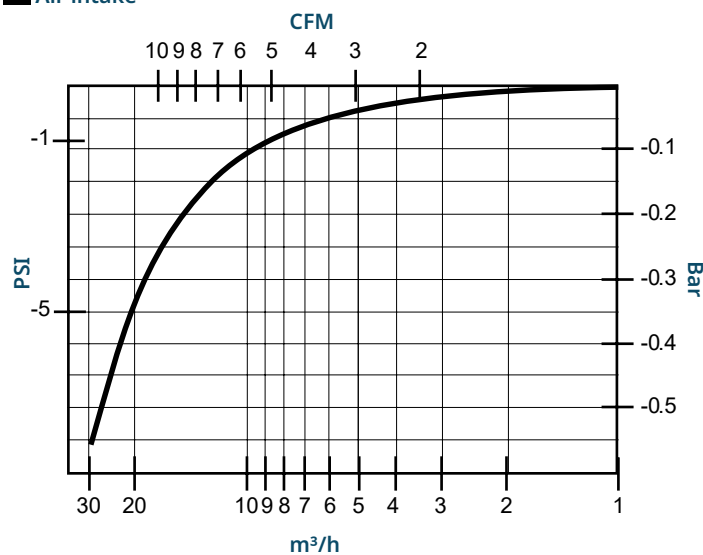
■ Air intake
