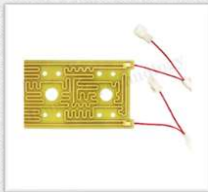
Epoxy Resin Heater
