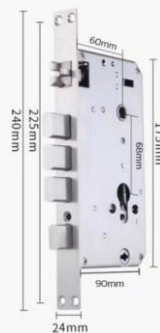
6068 Lock Body
