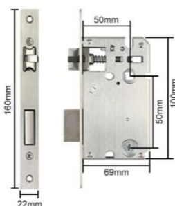
5050 Lock Body
