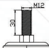
Threaded stem
