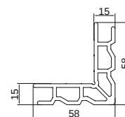
HW55T-K15/ THK. 2.6mm - 1.672 Kg/m
