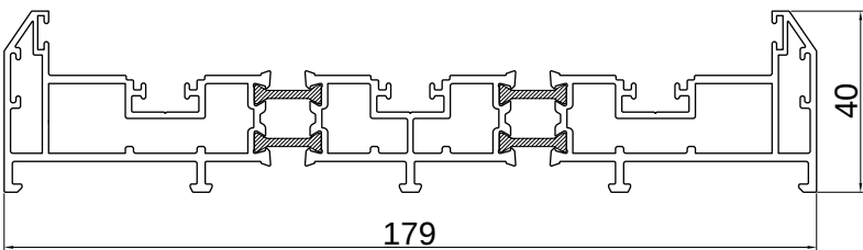
HW125T-F34/ THK. 1.4-1.8mm - 3.105 Kg/m
