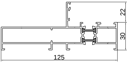
HW125T-F33/ THK. 1.4mm - 1.665 Kg/m
