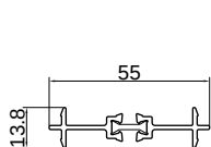
HW55T-C08/ THK. 1.4mm - 0.489 Kg/m
