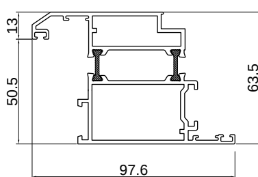
HW55T-S21/ THK. 1.8mm - 2.099 Kg/m
