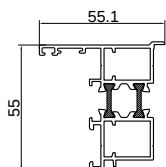
HW55T-M12/ THK. 1.4mm - 1.097 Kg/m
