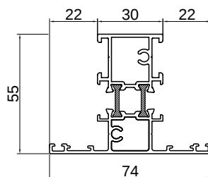
HW55T-T11/ THK. 1.4mm - 1.322 Kg/m
